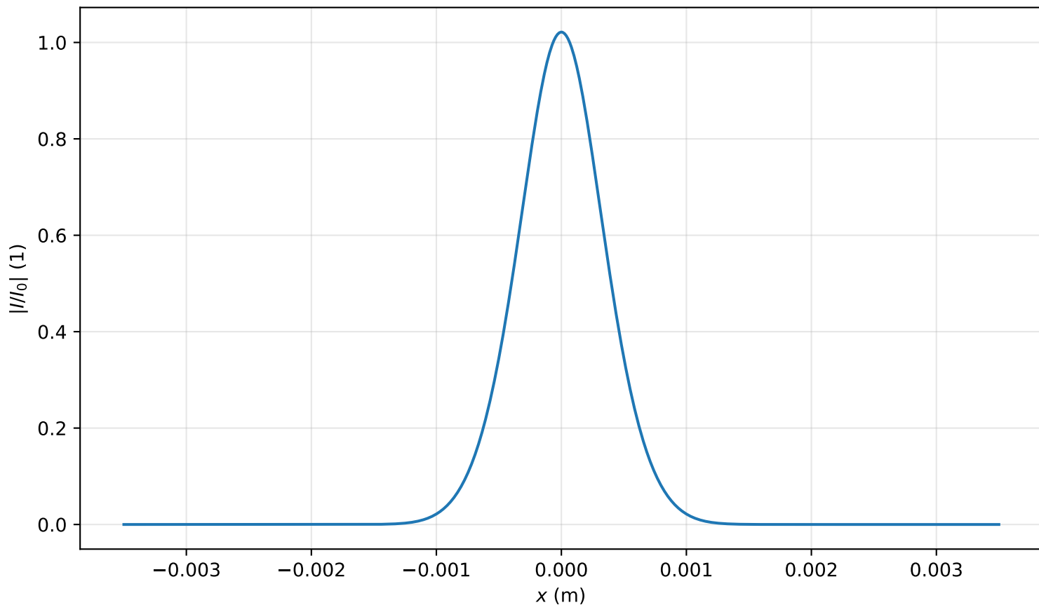
Intensity profile I(x, y = 0, z = 0.637m)/I_0 , P_{in}=0.4P_{cr} , artificial time
